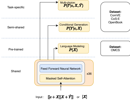
Figure 1: UNION Architecture
