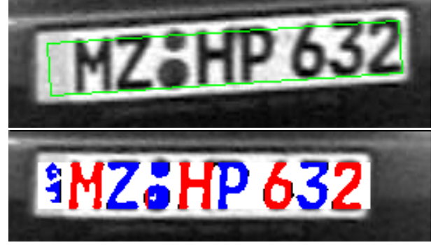
Figure 1: Original license plate image (with the detected license plate subimage framed) and the narrowest components found by the segmentation algorithm. Components are plotted in alternating colors/patterns. The segmentation boundaries are defined by the left and right edges of the narrowest components. Note that the segmentation algorithm successfully separated the letters 'H' and 'P'. However, the price is that it also cuts the stamp between the letters 'Z' and 'H' into two parts.
