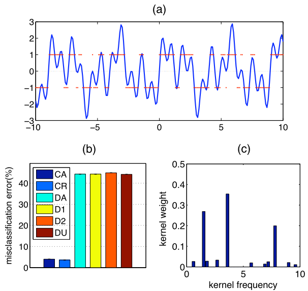
Fig. 2 (a) The function f(x) = \sin(\sqrt{2}x) + \sin(\sqrt{12}x) + \sin(\sqrt{60}x) used for generating synthetic data, along with \text{sign}(f) . (b) Misclassification percentages obtained by each algorithm. (c) The kernel frequencies found by the CA method
