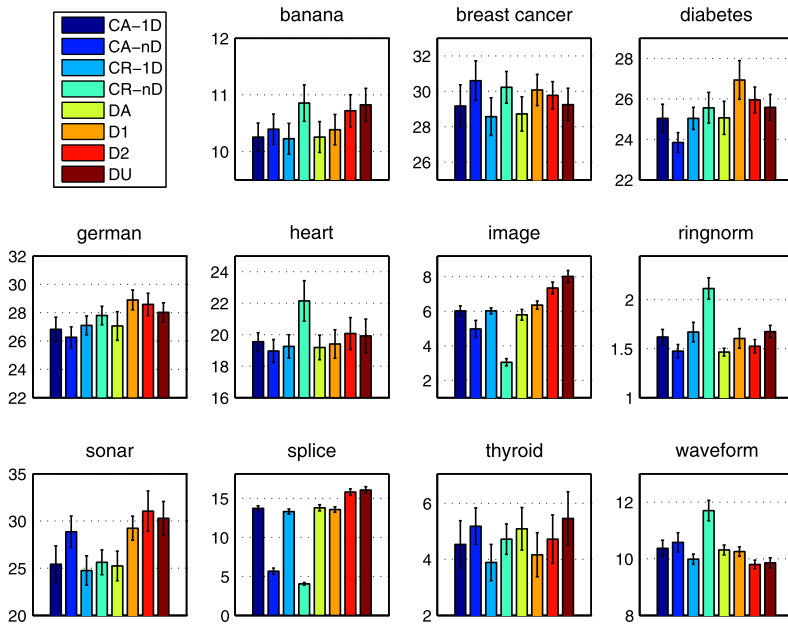
Fig. 8 Misclassification percentages obtained in 11 datasets
