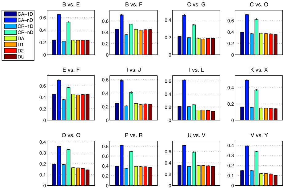
Fig. 7 Alignment values in different tasks of the UCI Letter recognition dataset
