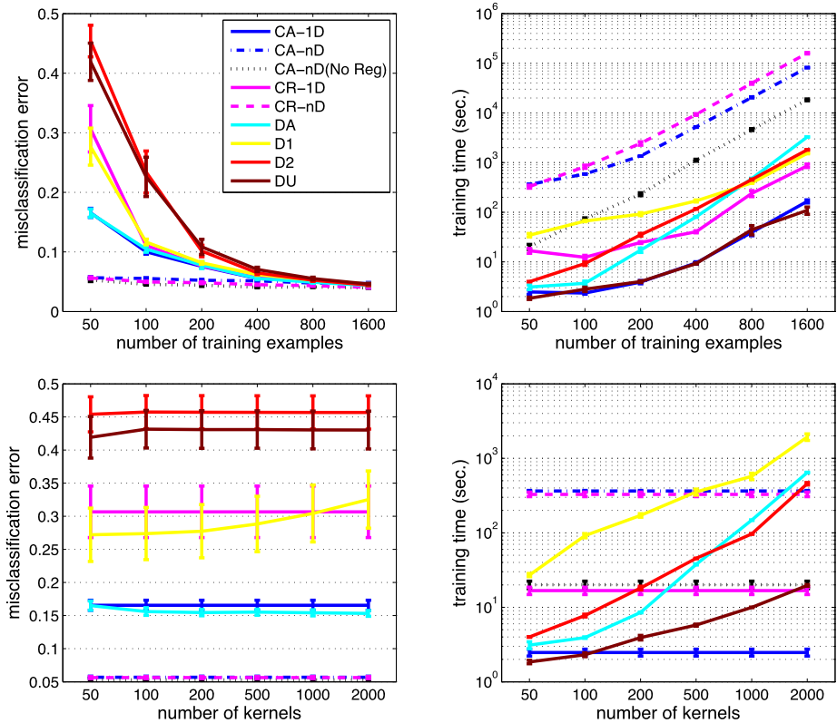
Fig. 4 Scalability of various methods with respect to the number of training examples ( top ) and the number of kernels ( bottom ). Results for the methods that search over a continuous range are included for comparison purposes in the bottom figures . Note that the curves of these methods are flat as they in fact do not rely on the provided finite kernel sets
