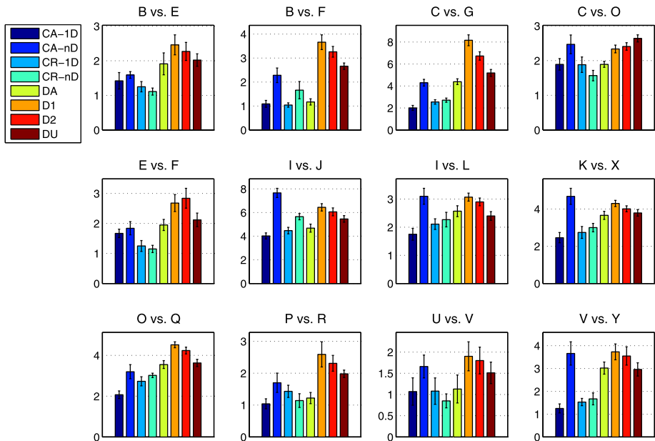
Fig. 6 Misclassification percentages in different tasks of the UCI Letter recognition dataset
